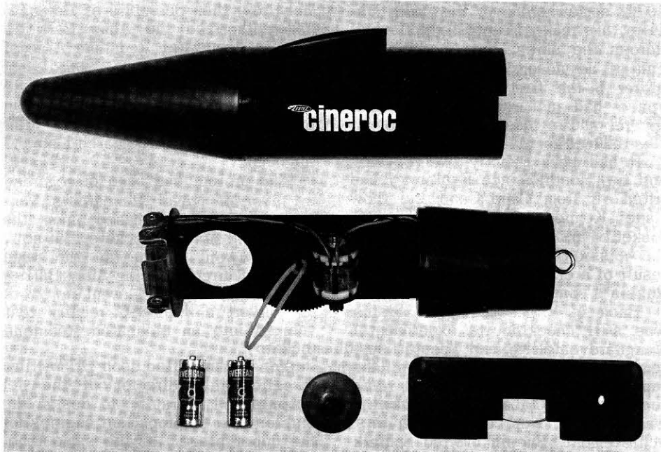
These are the components of the rugged, all-plastic Estes CINE-ROC. At top is the nose cone with the mirror hood, and right below it is the camera proper. The two PFB-2 batteries, drive pulley, and Flight-Pak are at the bottom.
