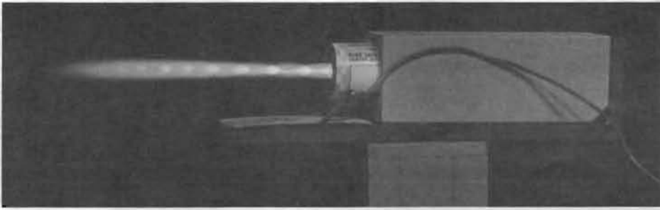
"Mach diamonds" are clearly visible in this photo of a night-time static firing. Quality testing for performance and safety goes on constantly at our motor production facility.
